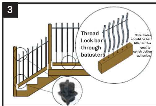
3 Install balusters
