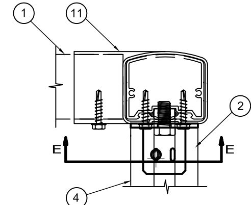
DETAIL 'B' SQUARE TOP CORNER
